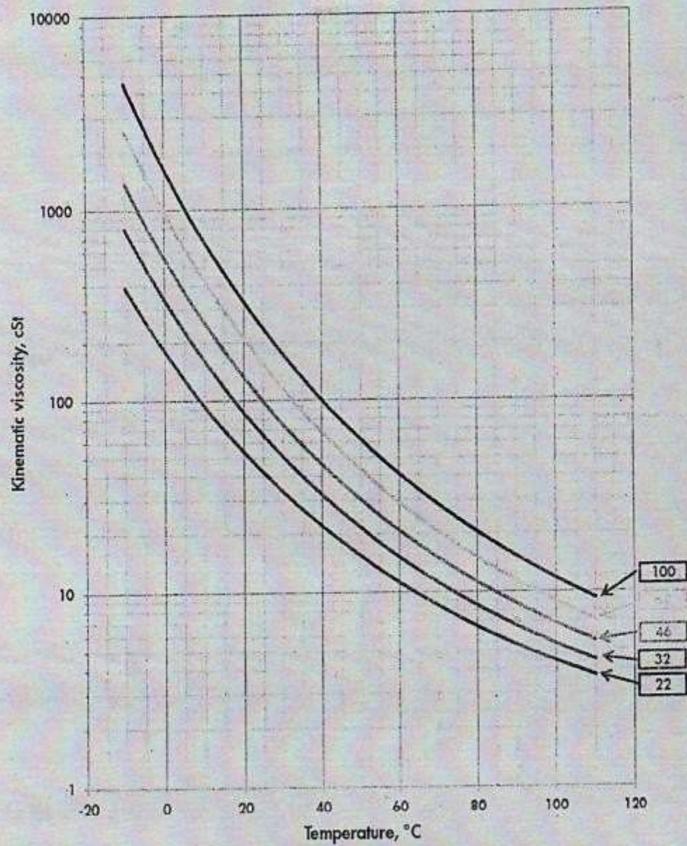
Viscosity - Temperature Diagram for Shell Tellus S2 MX
