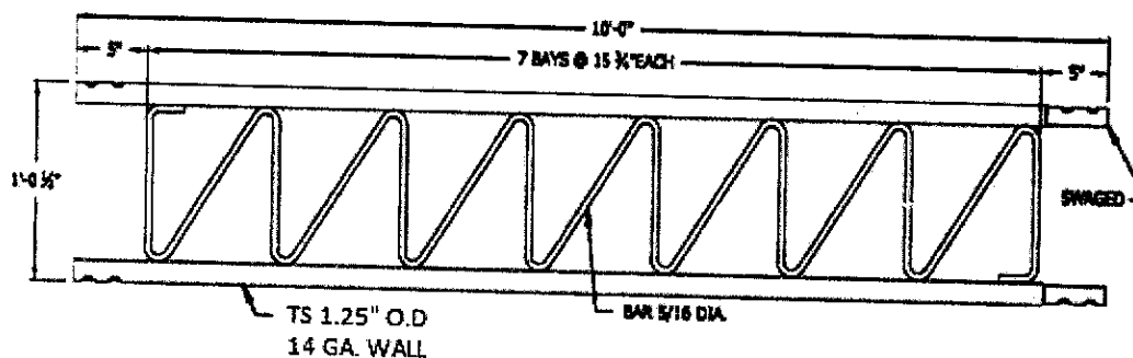
Lower Section of Tower (Min Approx. Weight 18 Kg)
