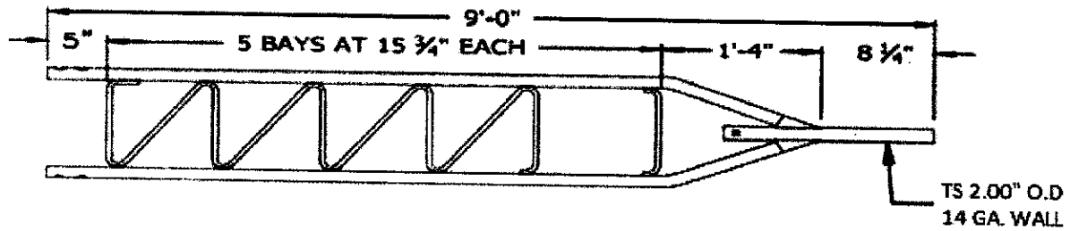
Upper Section of Tower (Min Approx. Weight 18Kg)
