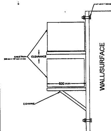
ANNEX "C" CABLE TRAY SUPPORT TYPE "B"
