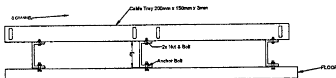
ANNEX "D" CABLE TRAY SUPPORT TYPE "C"
