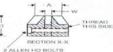
Dimensions of Standard Dumbbell Dies A (Metric Units)
