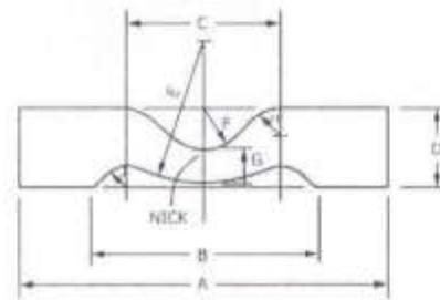
DIE B (ISO/34 CONFIGURATION)
