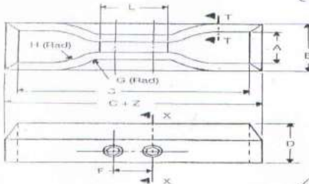
Dimensions of Standard Dumbbell Dies A (Metric Units)
