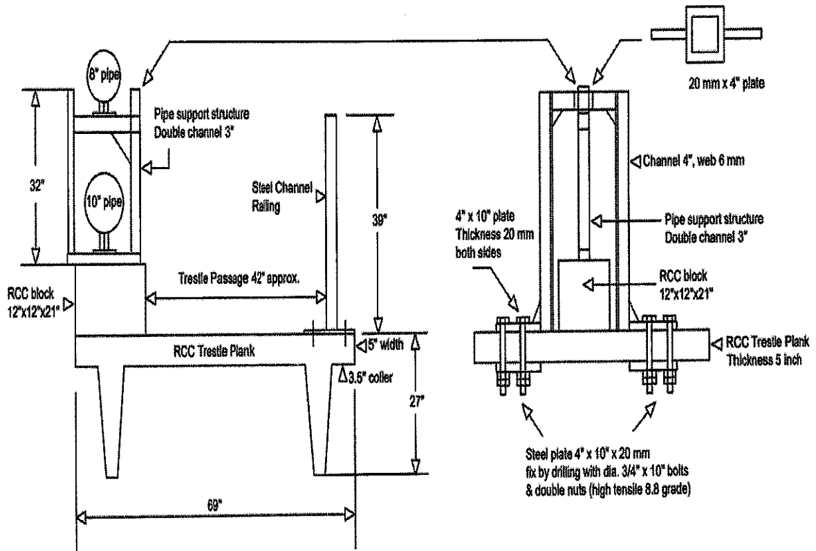
Fabrication & installation of support structure for LPG pipe support at Trestle
