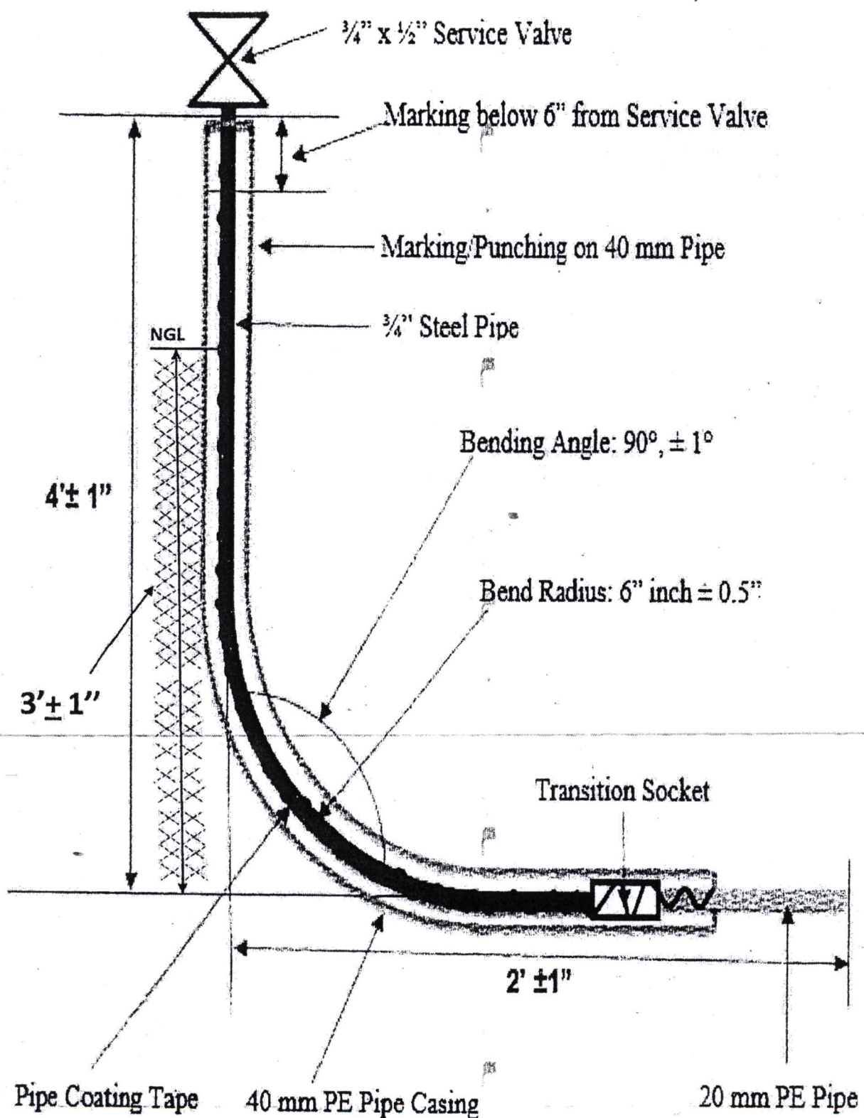
Figure 2: Sketch of Riser Assembly
