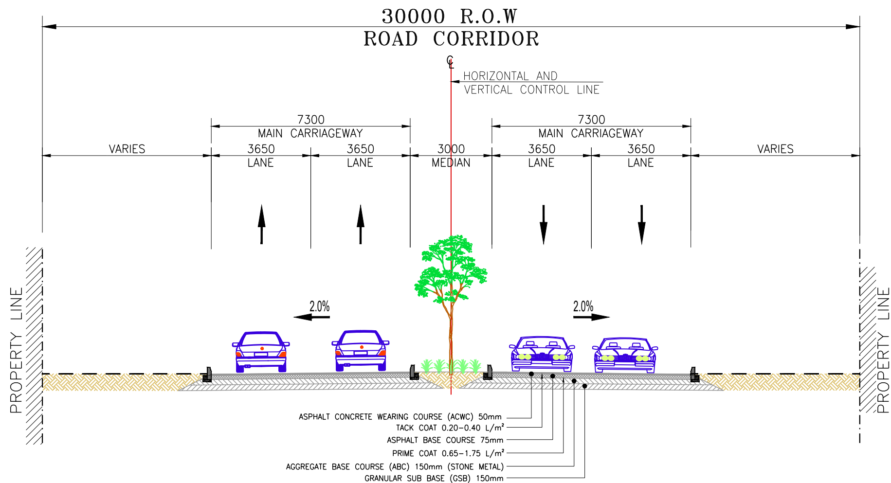
TYPICAL CROSS SECTION B-B
