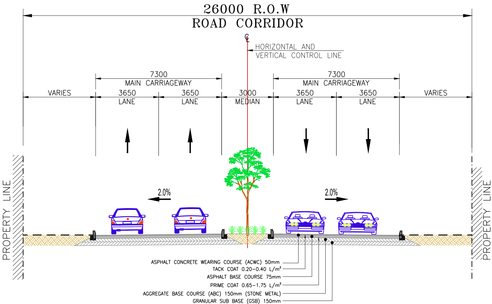
TYPICAL CROSS SECTION A-A
