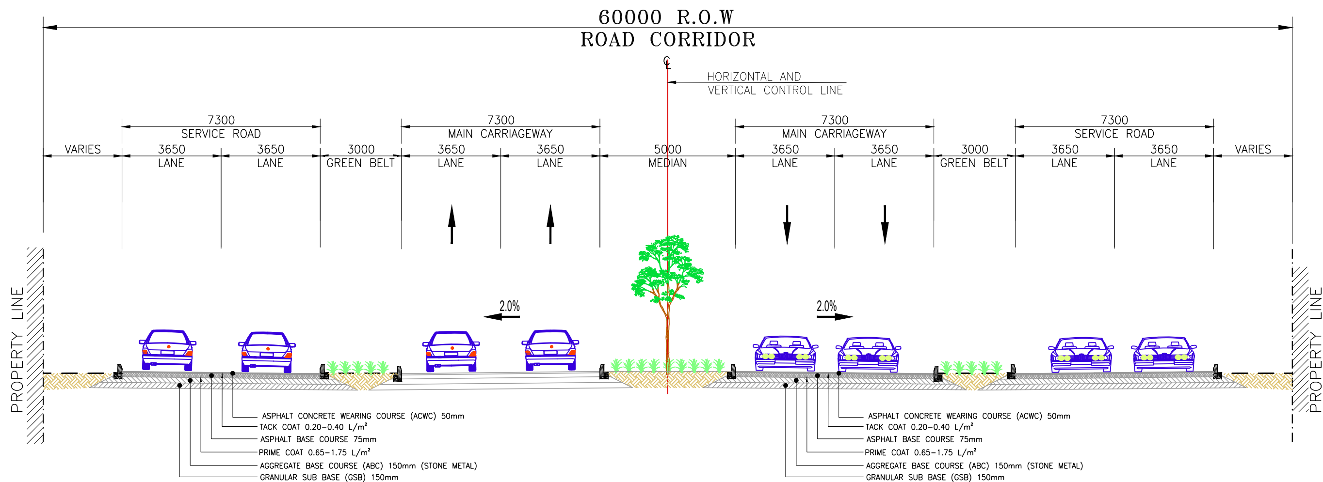
TYPICAL CROSS SECTION B-B
