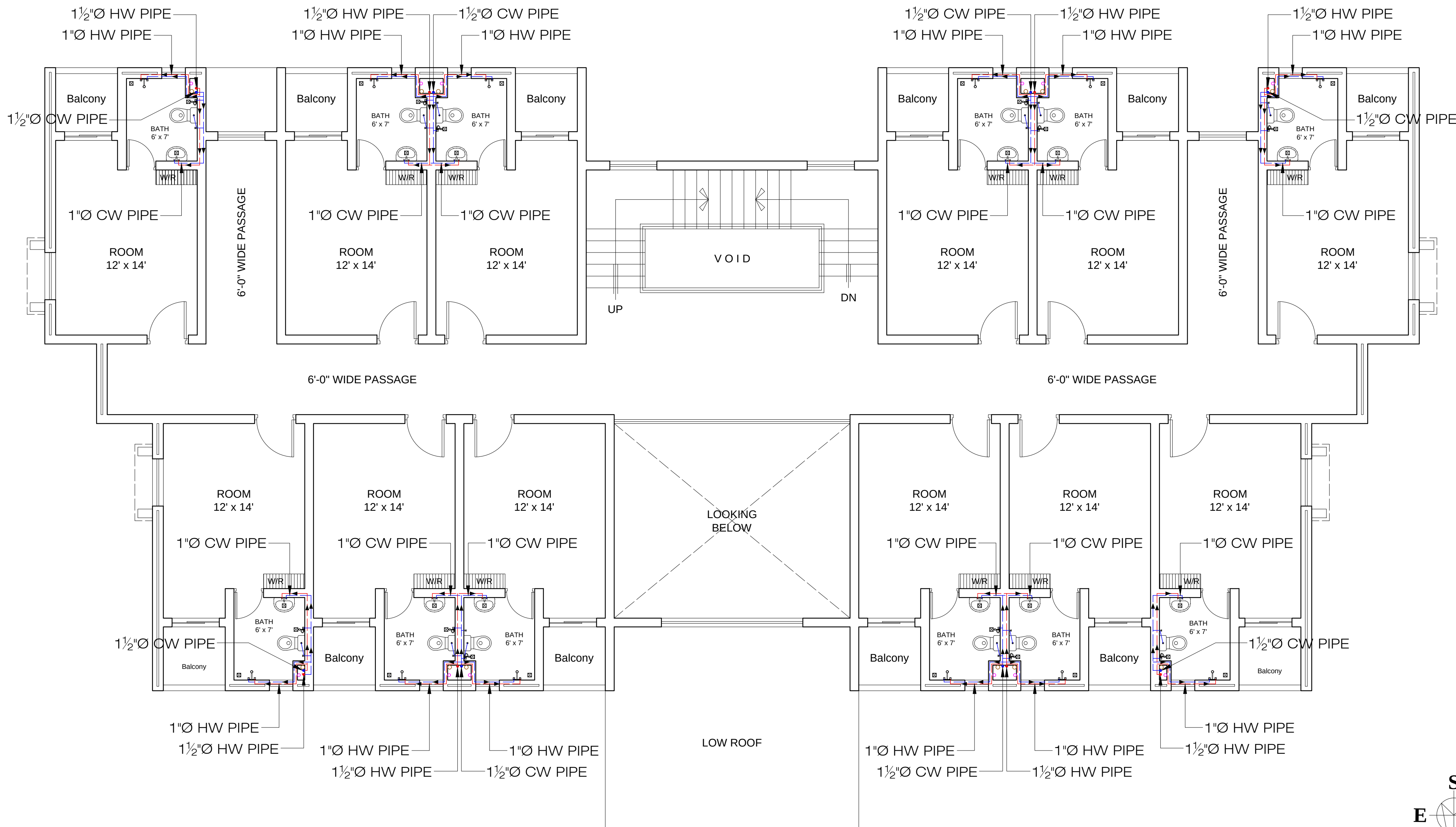
FIRST FLOOR PLAN Water Supply
