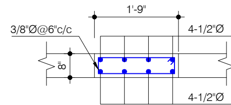
Section of C.B.1
