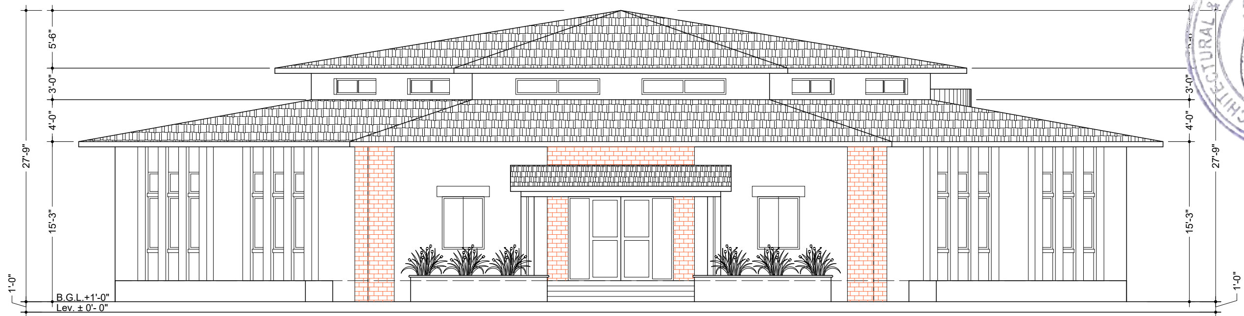
FRONT ELEVATION - 01
