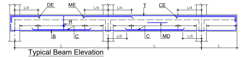
SCHEDULE OF ROOF BEAMS
