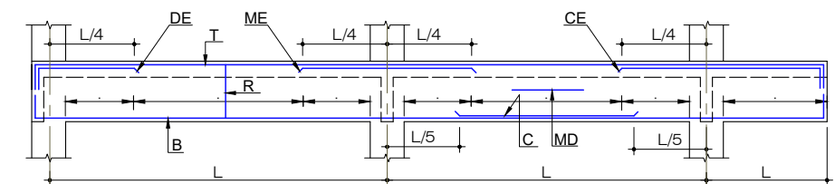
TYPICAL BEAM ELEVATION
