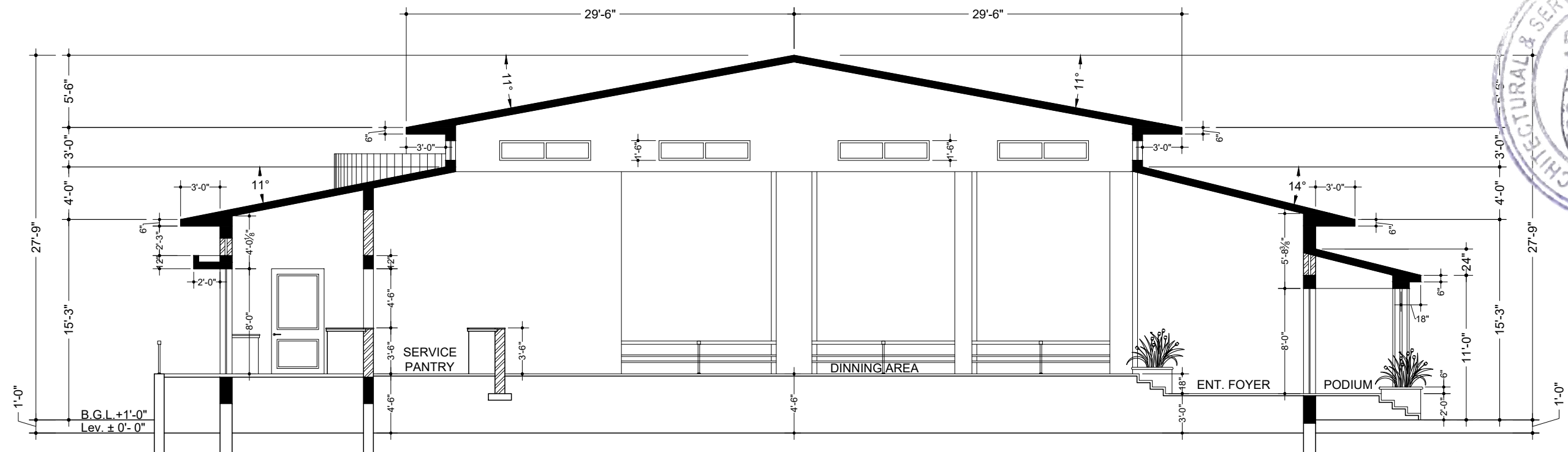
SECTION B-B
