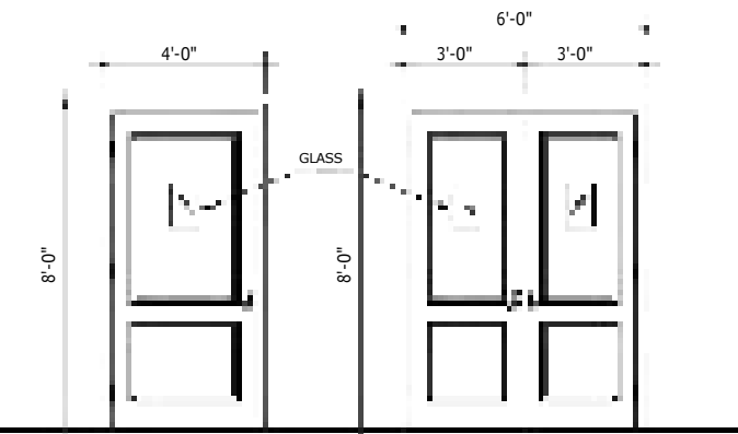
DOORS WITH GLASS SEMINAR HALL, VIDEO CONFERENCE HALL, HOSTEL ROOM & CLASS ROOM
