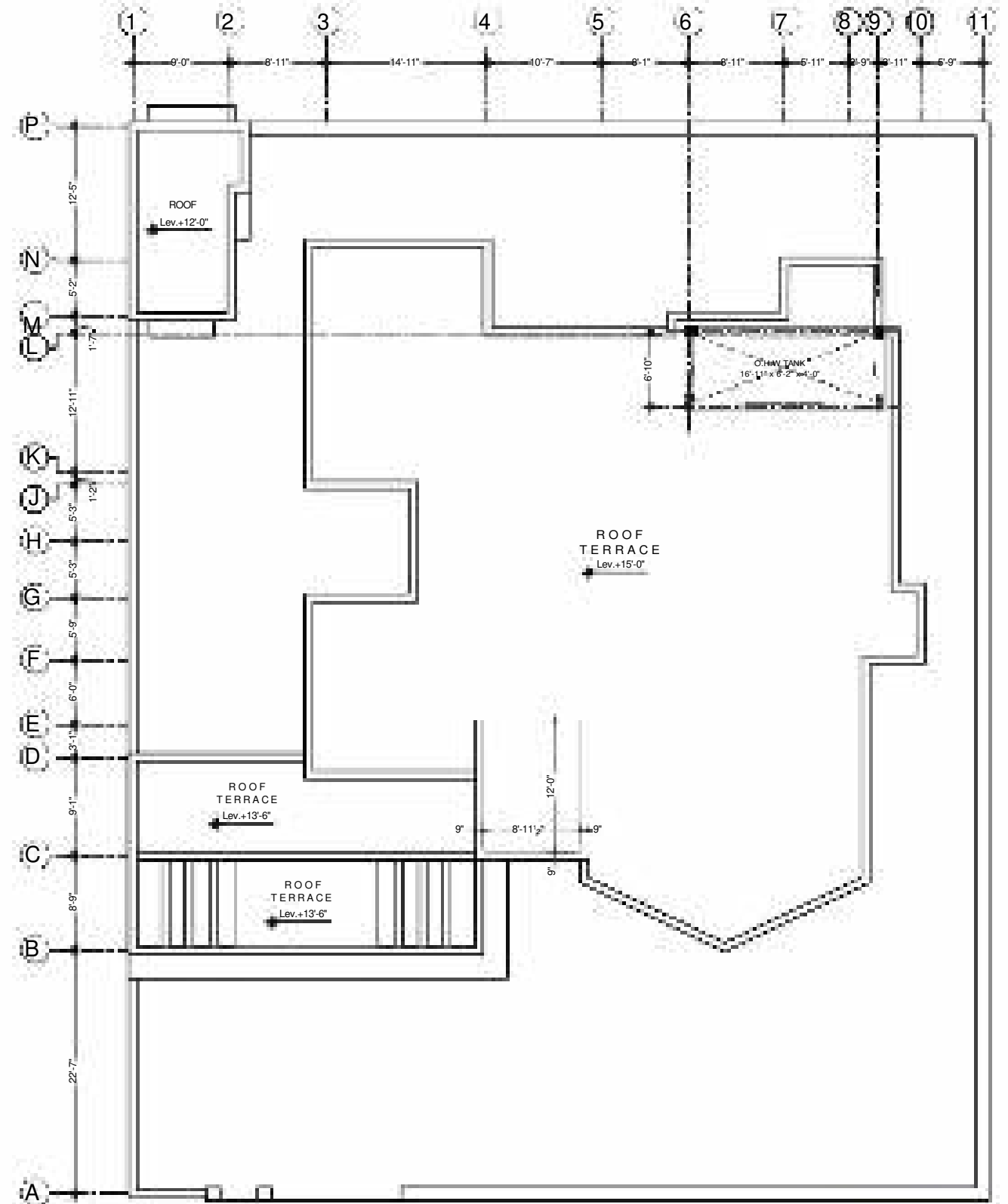
ROOF PLAN
