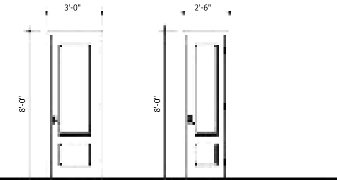
DOORS TOILET BLOCK & BATH ROOM
