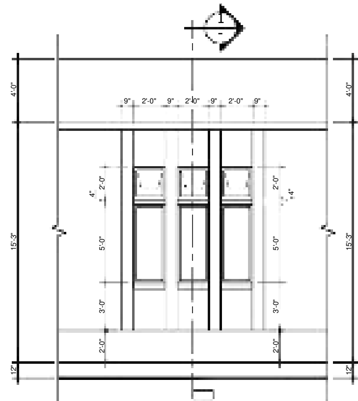
PART ELEVATION
