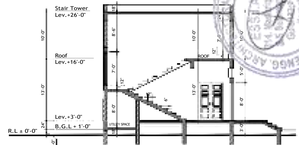
SECTION C-C
