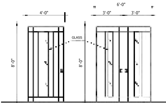
DOORS WITH GLASS SEMINAR HALL, VIDEO CONFERENCE HALL,
