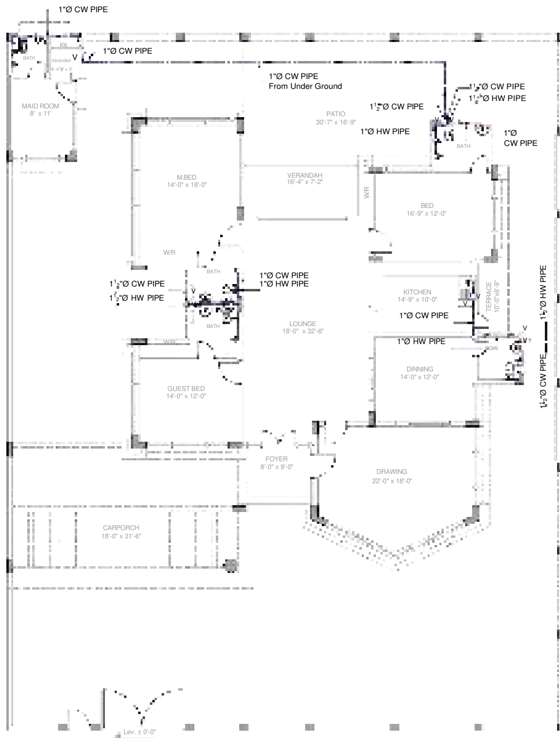
GROUND FLOOR PLAN Water Supply
