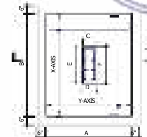
TYP. PLAN OF FOOTING
