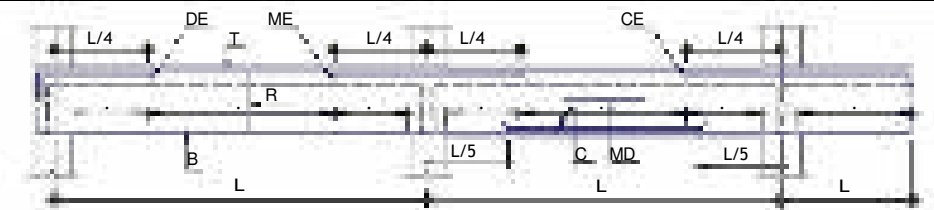
TYPICAL BEAM ELEVATION
