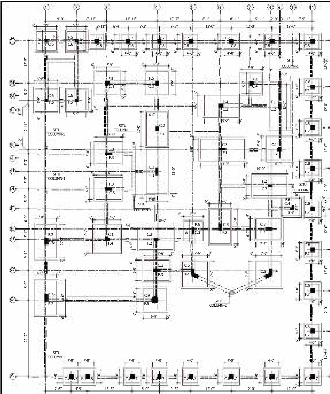
FOUNDATION PLAN
