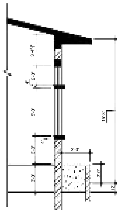
SECTION 1-1
