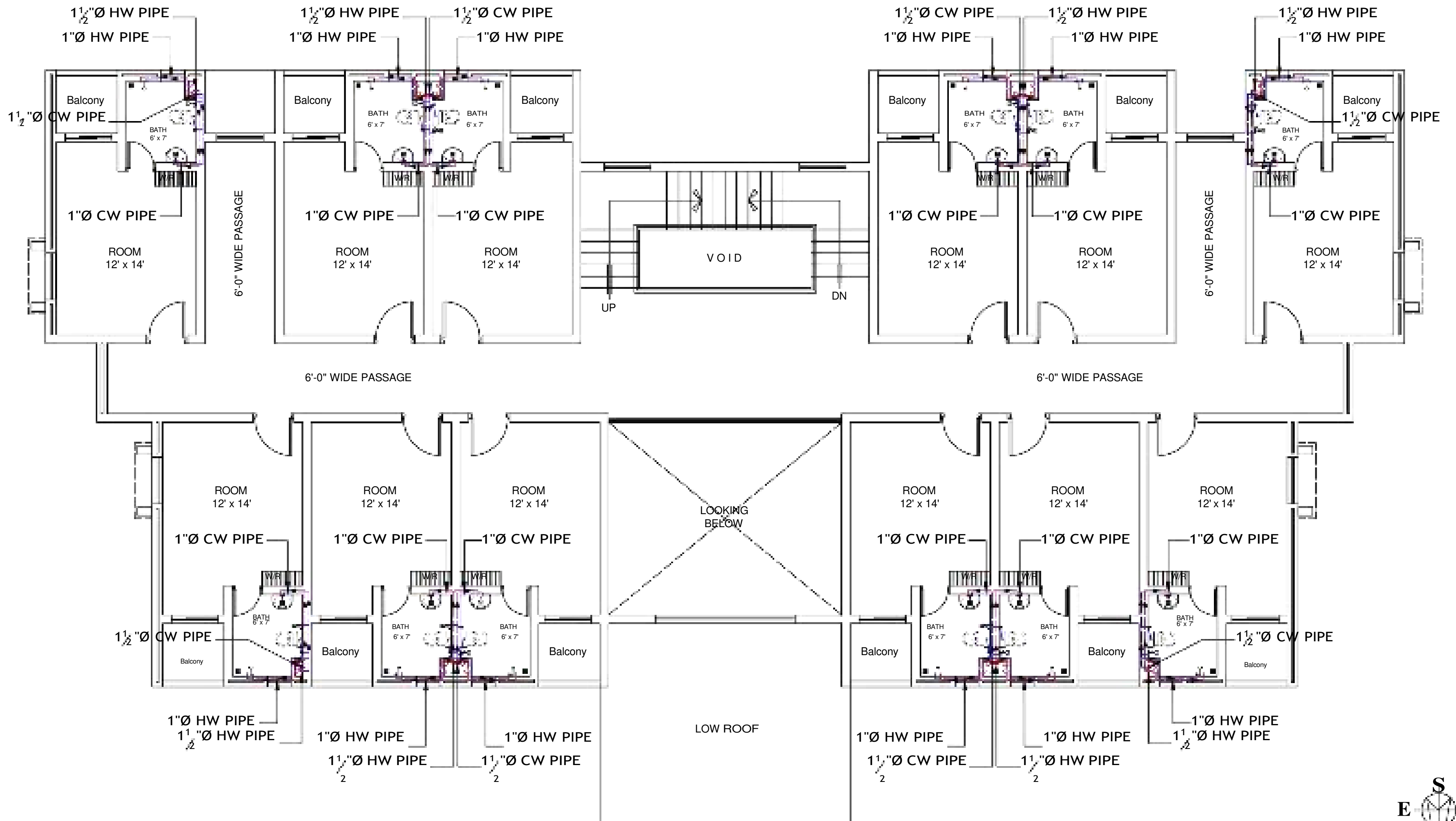
FIRST FLOOR PLAN Water Supply
