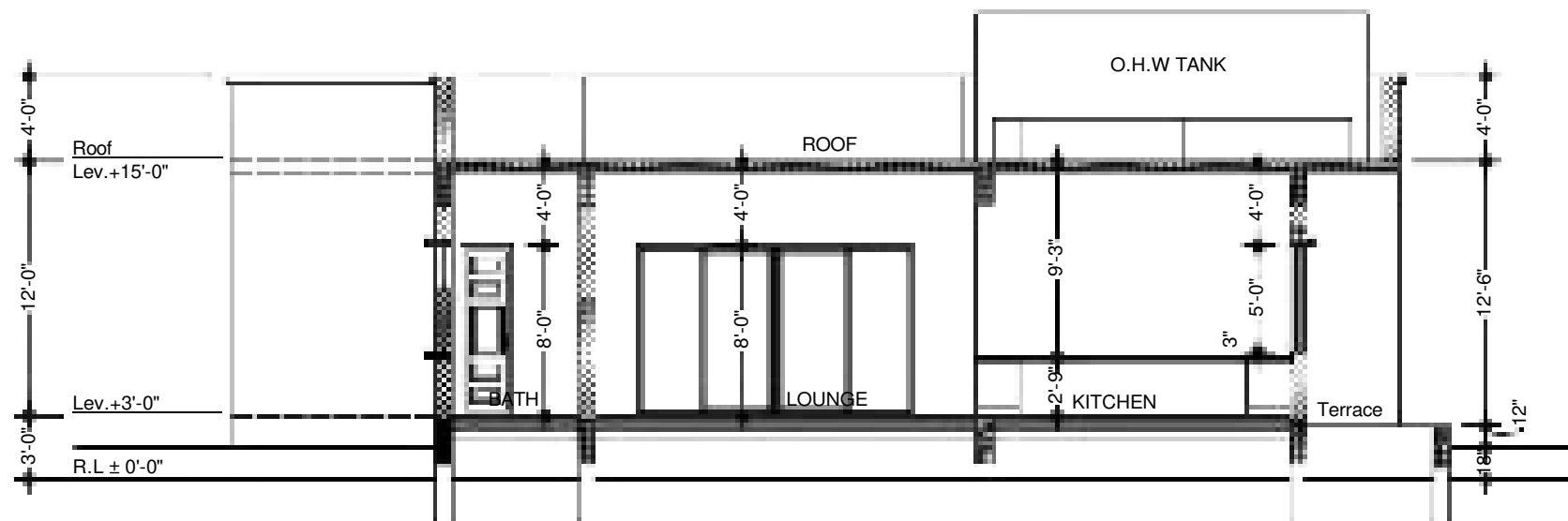
SECTION B-B
