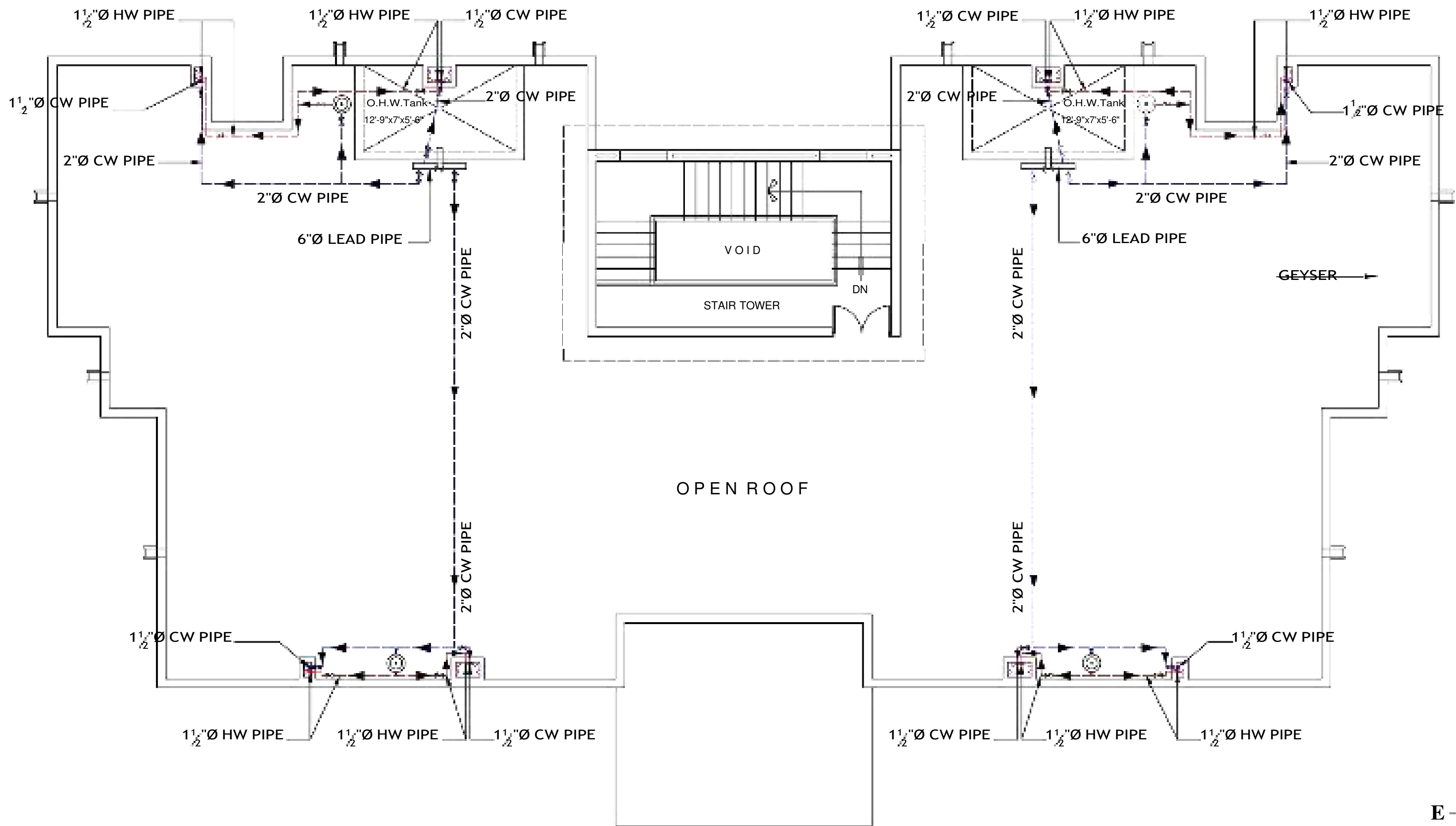
ROOF PLAN Water Supply
