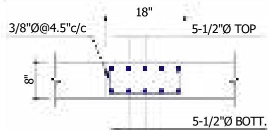
SECTION. OF C-B
