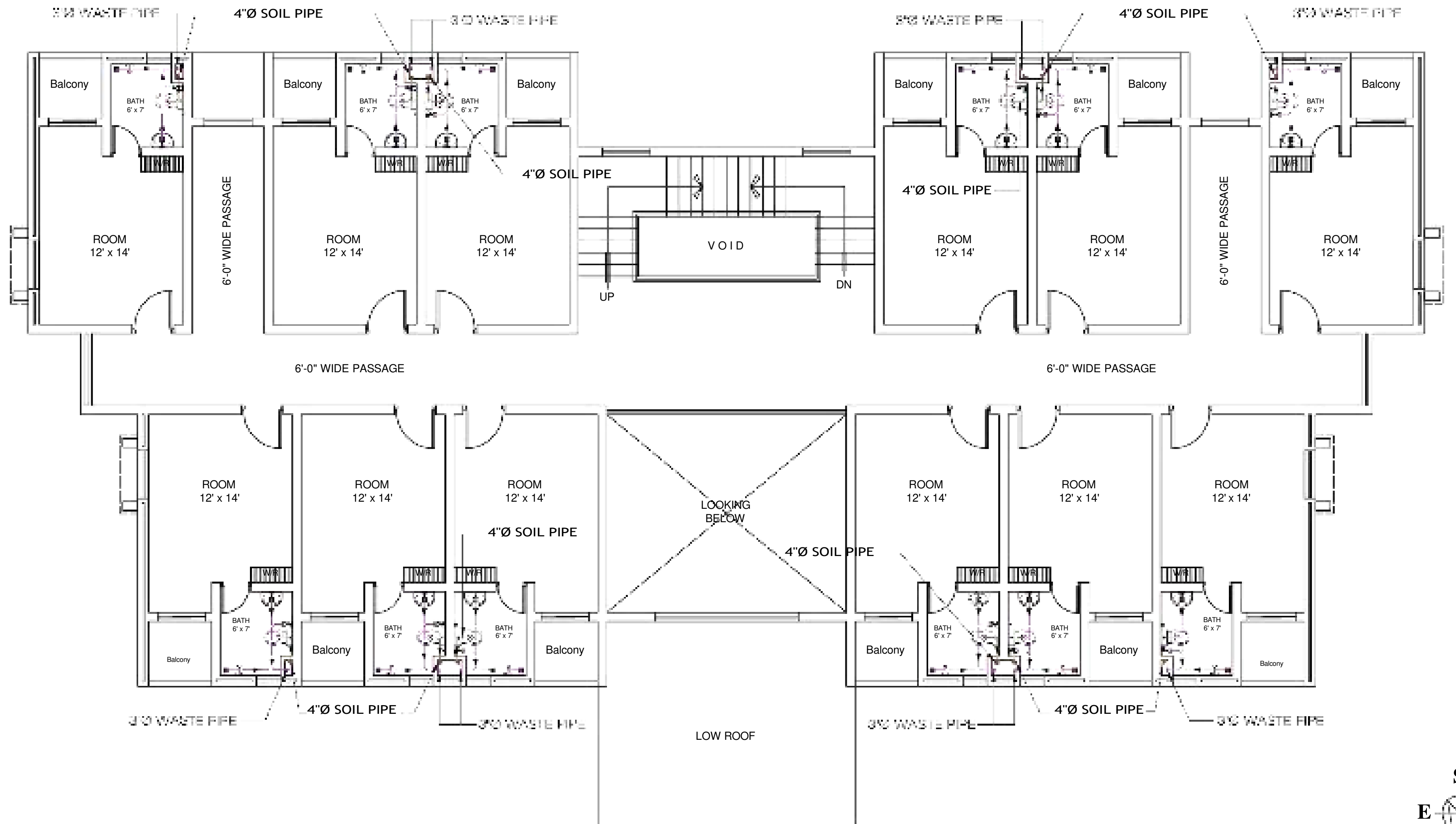
FIRST FLOOR PLAN Sewerage Layout
