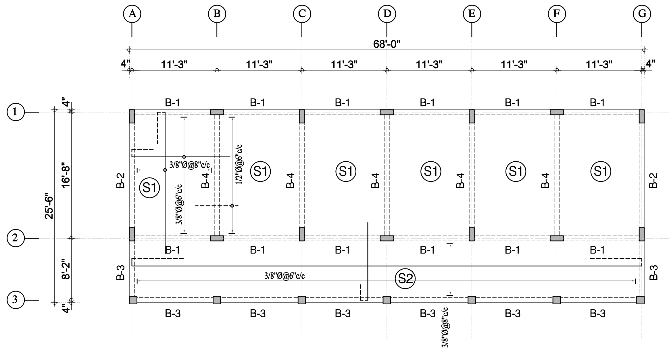
FRAMING LAYOUT PLAN
