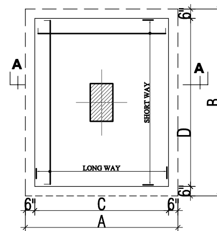
TYP. FOOTING PLAN
