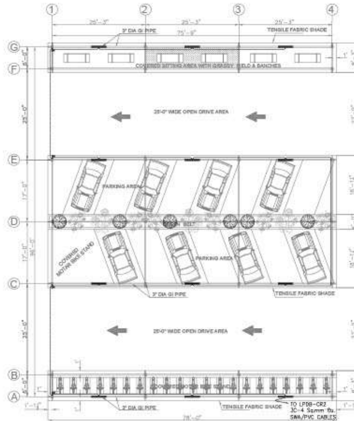
PARKING AREA PLAN
