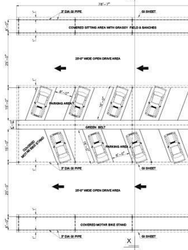
PARKING AREA PLAN
