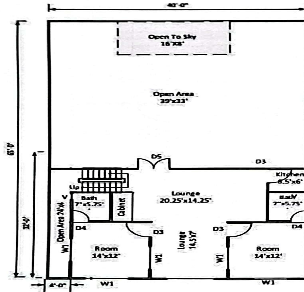
FIRST FLOOR LAYOUT PLAN SCALE N.T.S.
