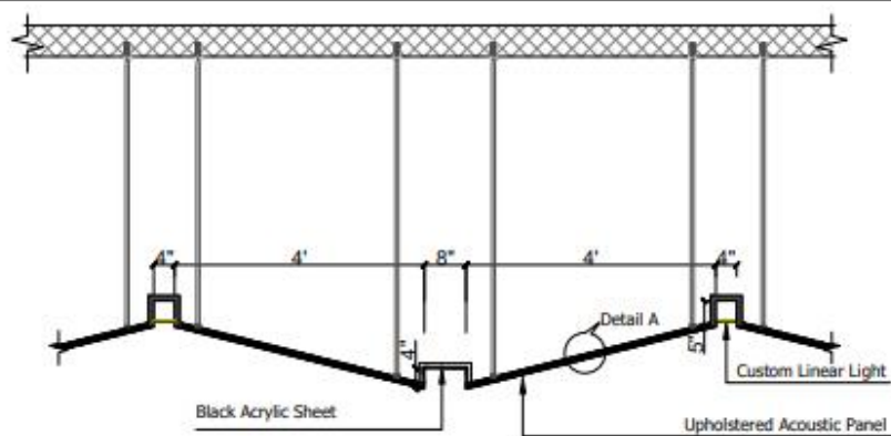
Ceiling Below Up Detail
