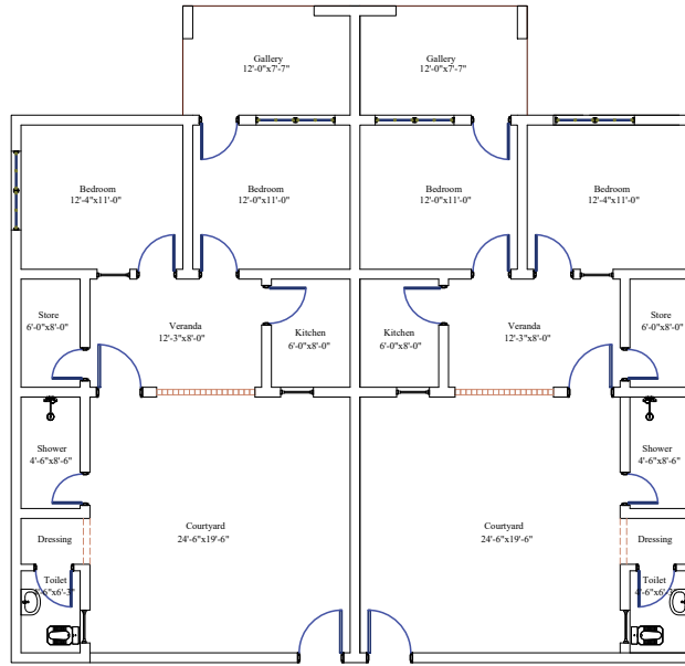
STAFF QUARTERS PROPOSED PLAN
