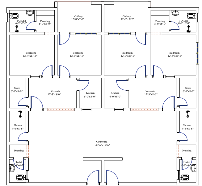
EXECUTIVE STAFF QUARTERS PROPOSED PLAN
