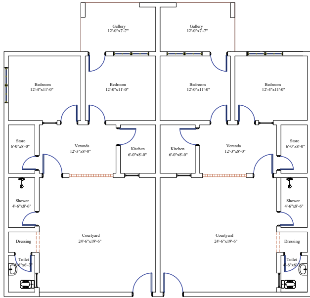
STAFF QUARTERS PROPOSED PLAN
