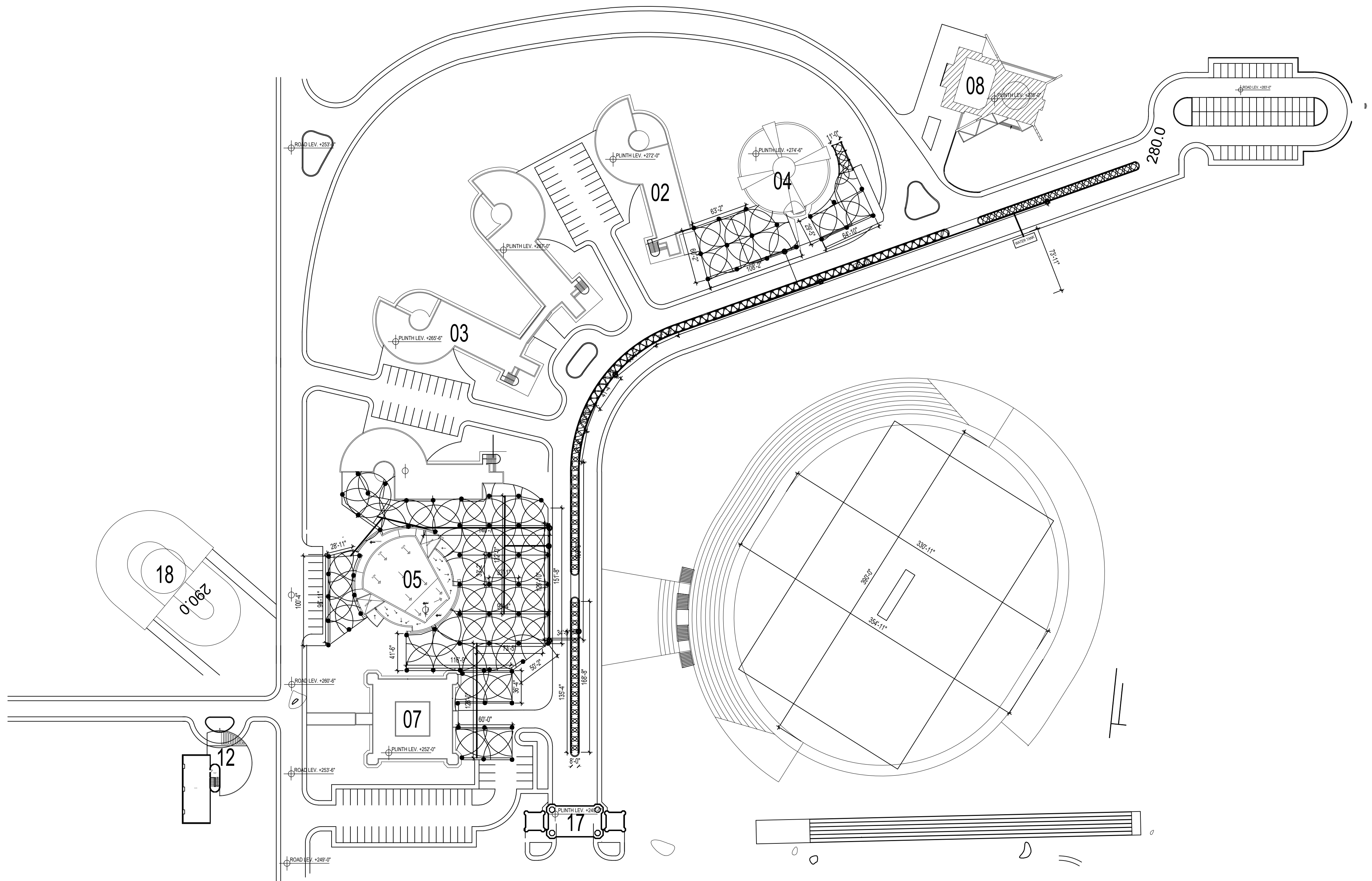
LAYOUT OF SPRINKLER SYSTEM IN LAWNS AND MEDIAN OF ROAD AT AROR UNIVERSITY SUKKUR-MAS-25-7-2026
