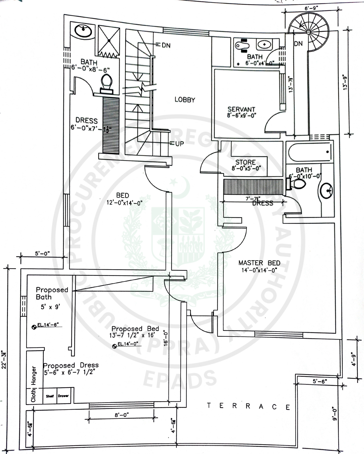
FIRST FLOOR PLAN AFTER ADDITIONAL BED ROOM NV - 09 to 23
