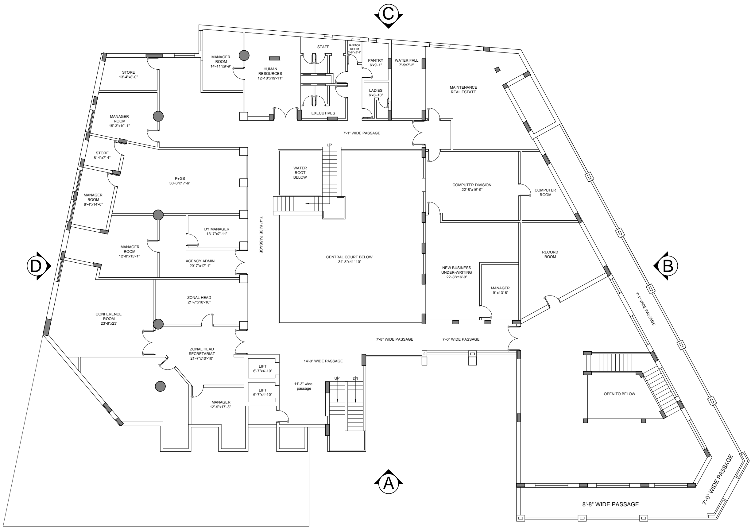
FIRST FLOOR
