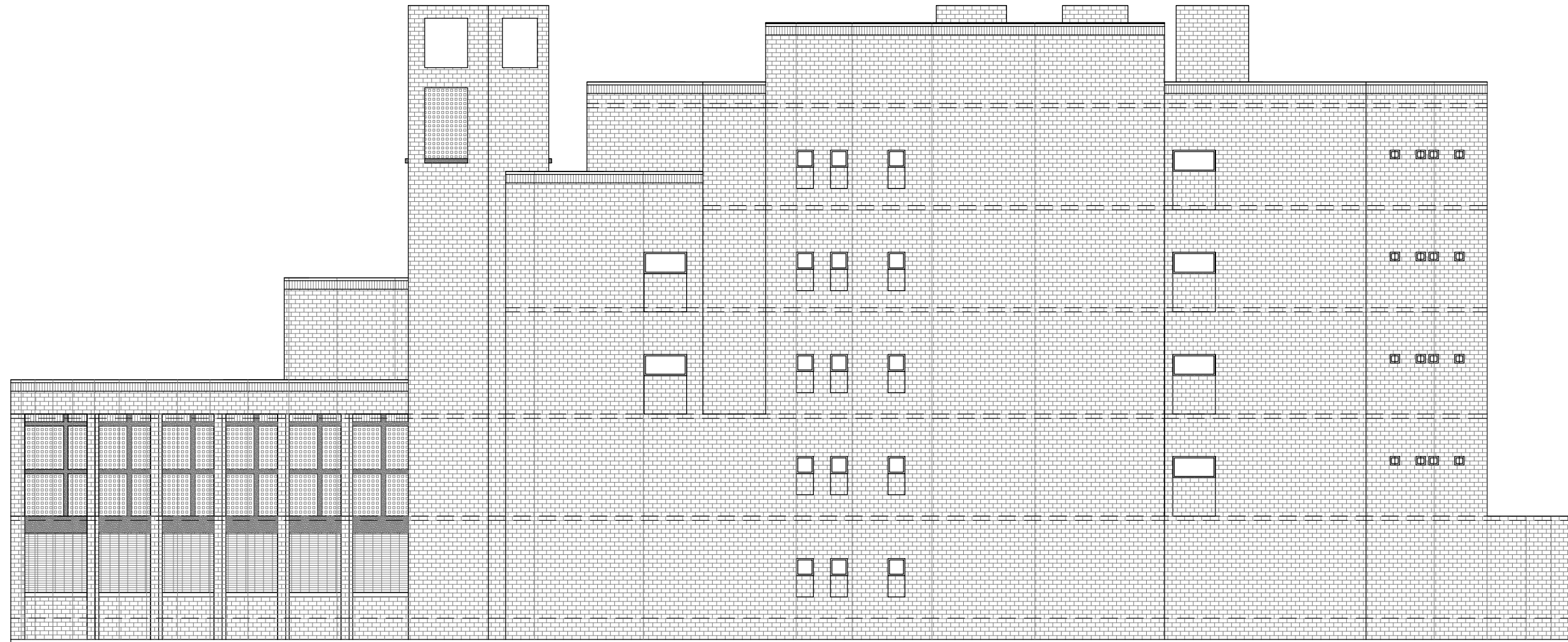
ELEVATION-C
