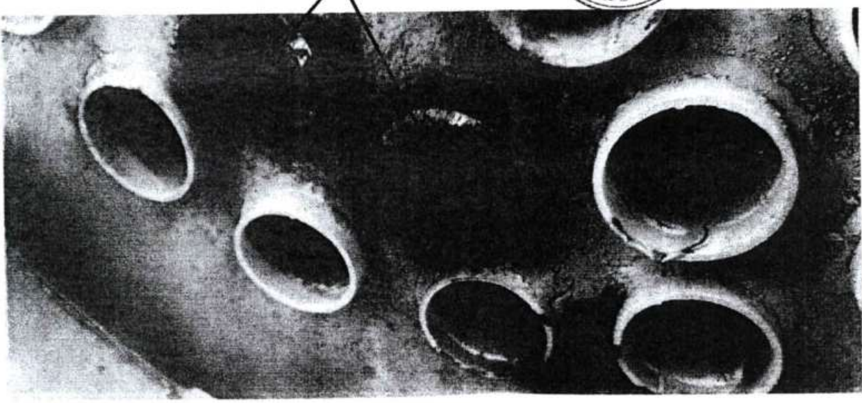
Leaked Heat exchanger pipes blocked bottom side
