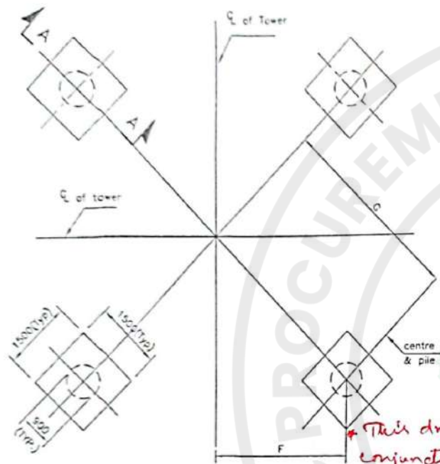
PLAN AT TOP OF PILE CAP PAD
