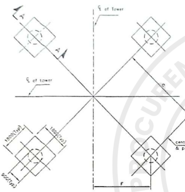
PLAN AT TOP OF PILE CAP PAD
