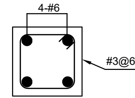
C-1 (9" X 9")
