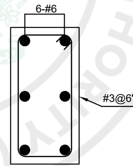
C-1 (9" X 18")
