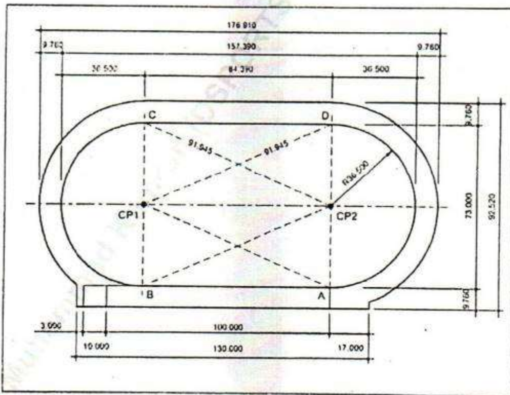
Figure 2.2.1.1a - Setting out plan and dimensions of the 400\text{m} Standard Track (Dimensions in m)
