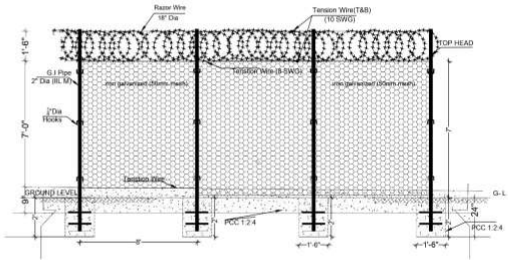
Elevation of Boundary Wall / Fence Wall
