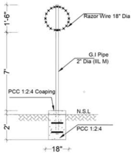
X- Section of Mesh Fence (B-B)
