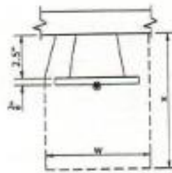
BACK POCKET DETAIL-6
