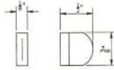
HOOK DETAIL-3
