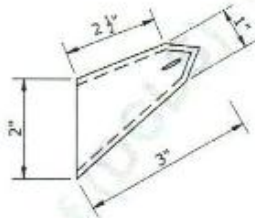
INNER FLAP DETAIL-2
