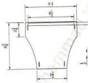
BIB DETAIL-6
