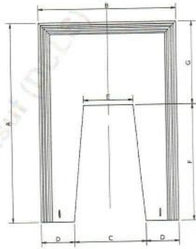
COLLAR DETAIL-7
