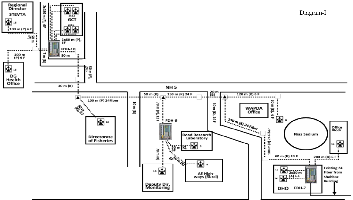
Layout Diagram of Optical Fiber Cable Network for GPoN Connectivity from District Health Office (DHO) MSAG at Hyderabad.
