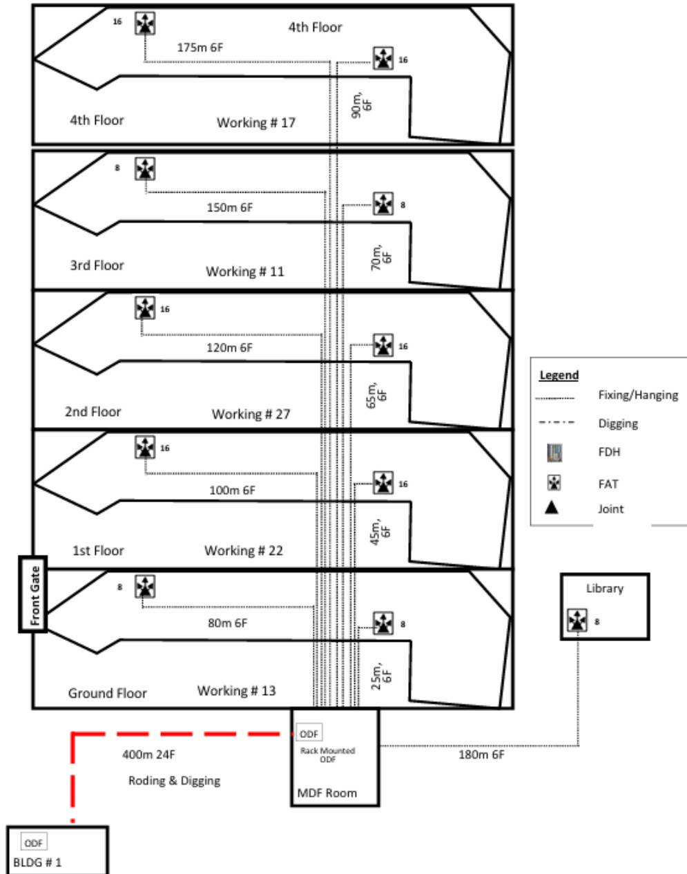
Layout Diagram for Laying of GPoN Based OFC Network at Old KDA Building
