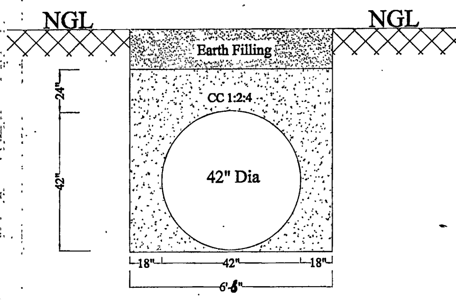
SECTION F-F MP-206(42" Dia)
