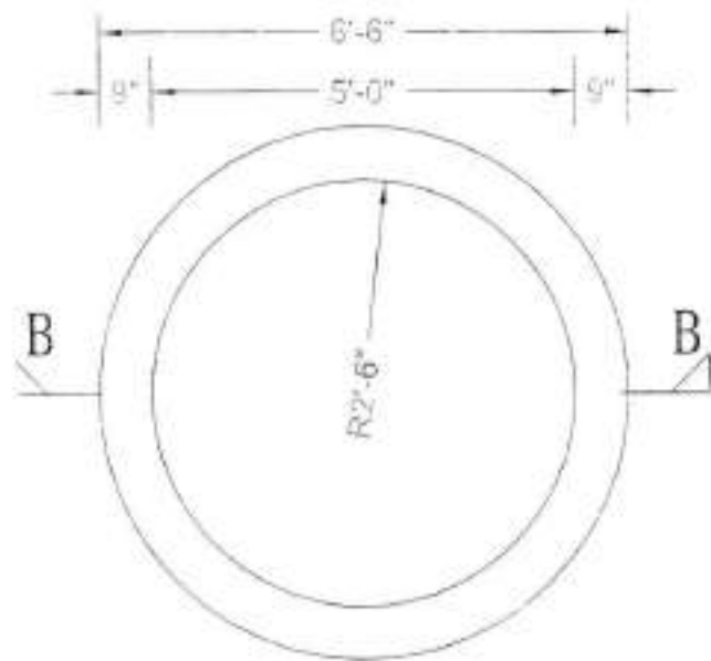
SOAKAGE PIT PLAN
