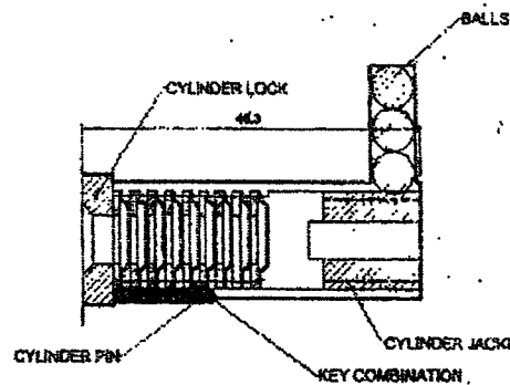
CYLINDER INTERIOR
