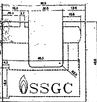
LOCK BODY EXTERIOR ELEVATION
