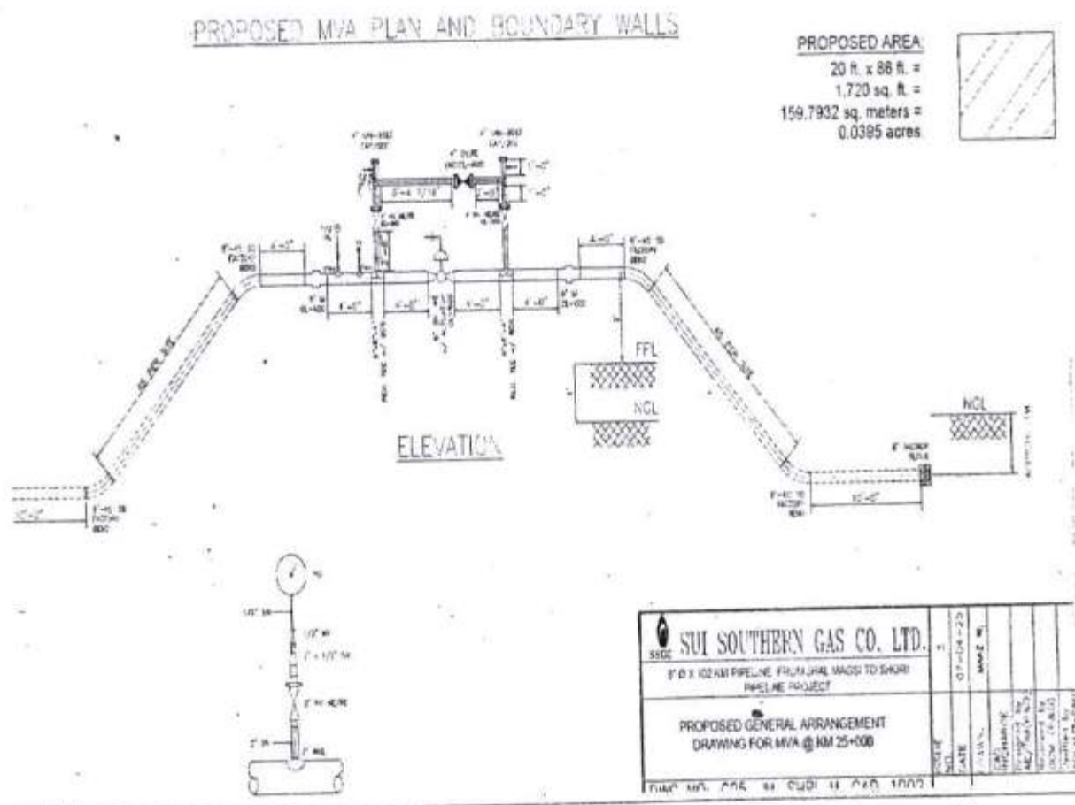
Figure 4. Schematic MVA-25
