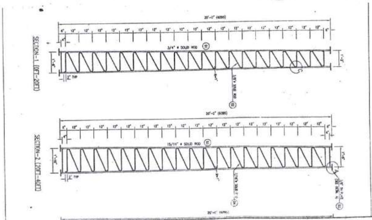
Figure 10, Schematic 2-Tower
