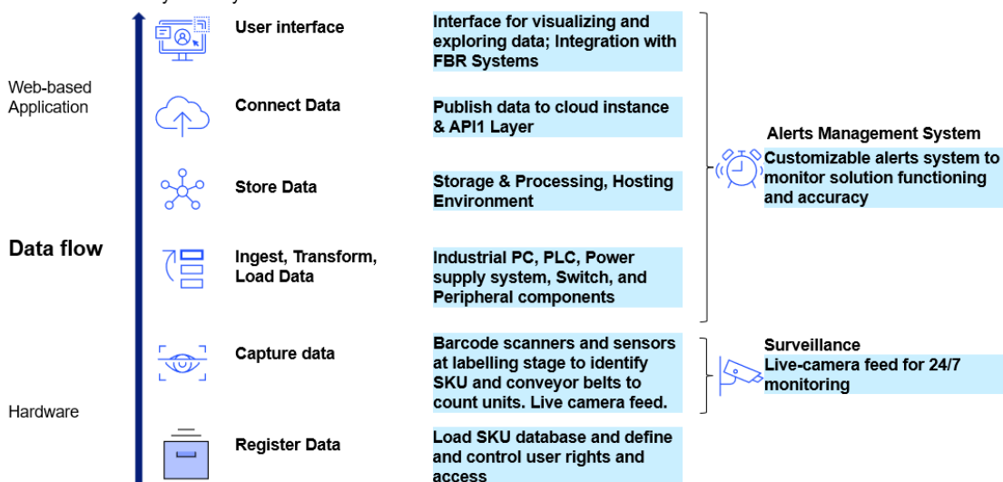
Figure A. High-level overview of technical architecture
