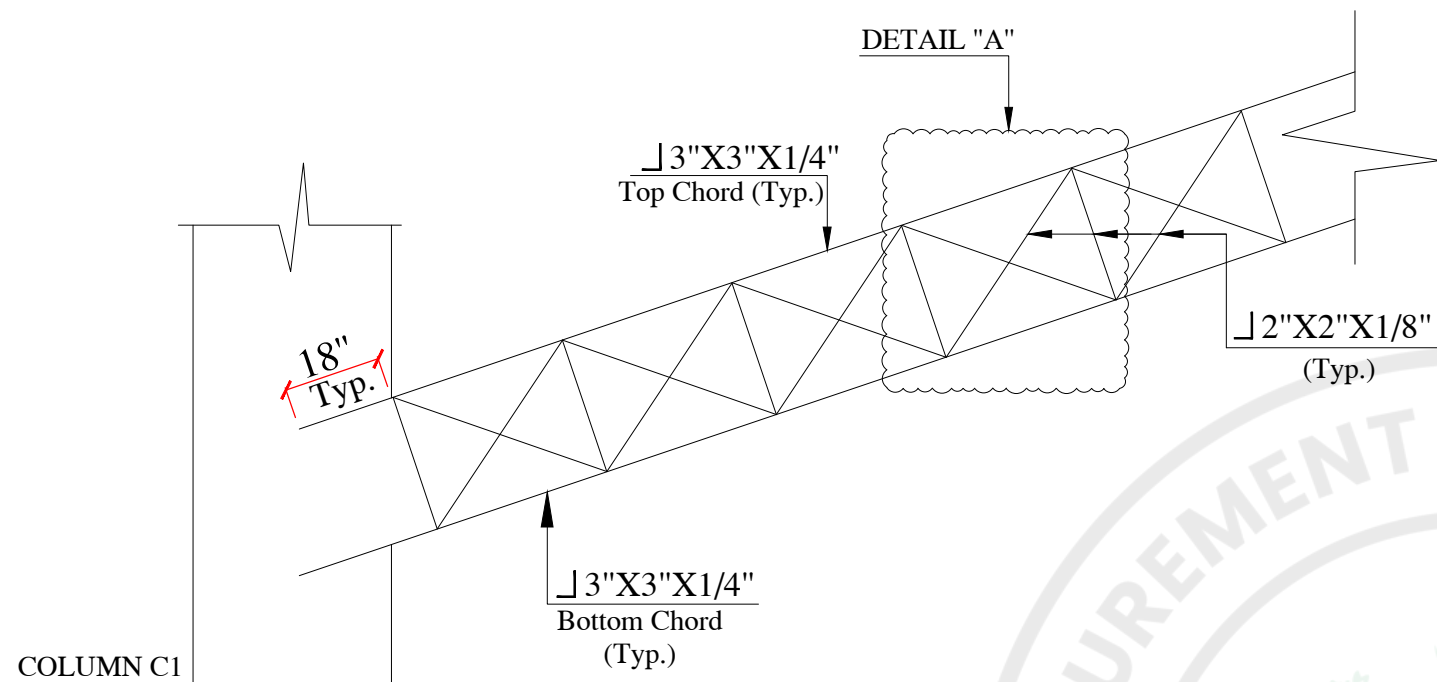
TYPICAL ELEVATION OF TRUSS
