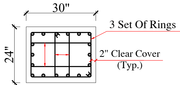
C1 (Gate Column)
