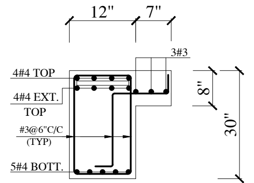
(LEDGE DETAIL)
