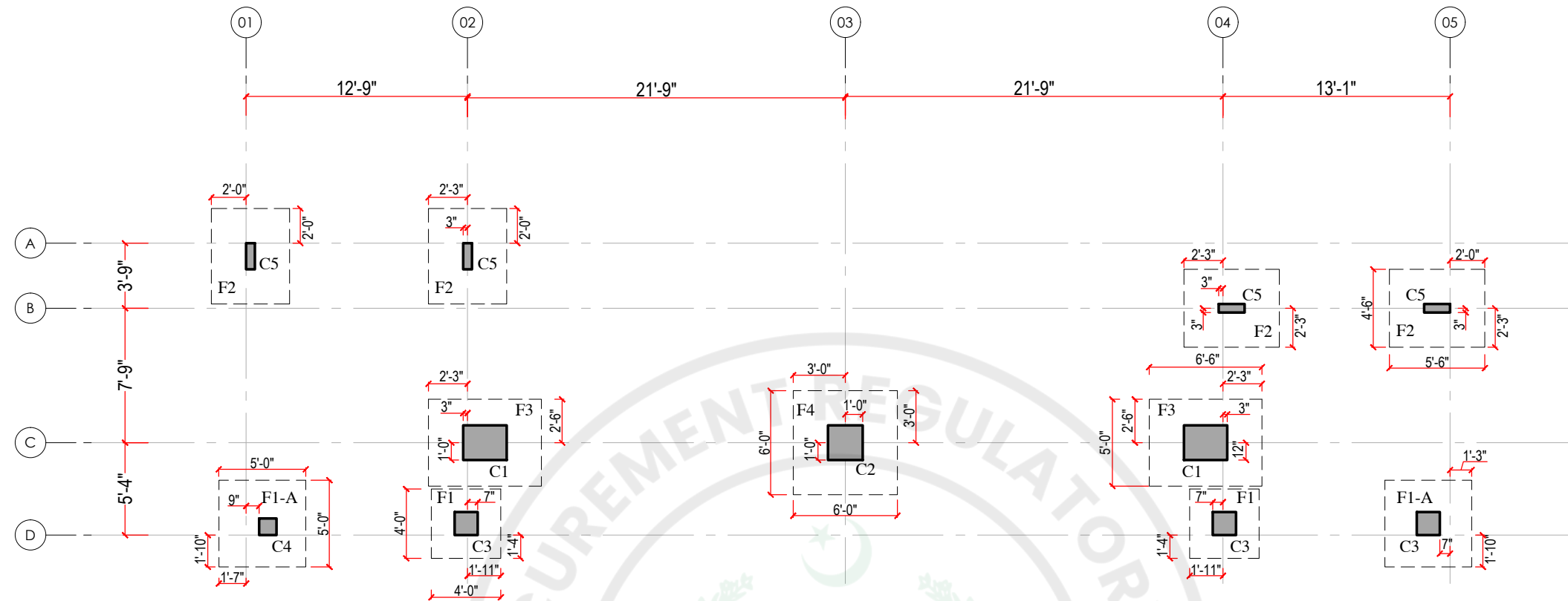
FOUNDATION PLAN
