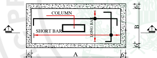
TYP. PLAN OF FOOTING
