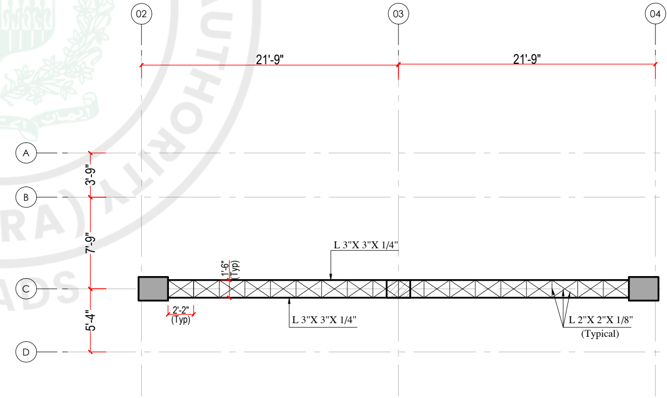
STEEL TRUSS PLAN
