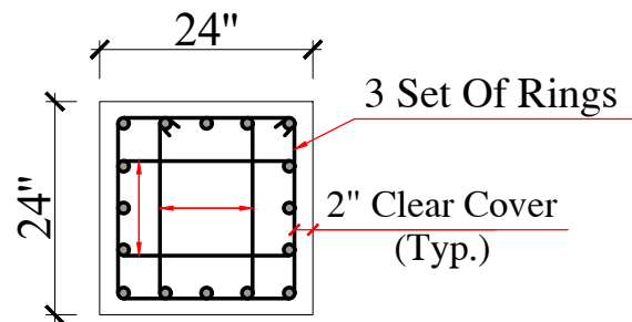
C2 (Gate Column)
