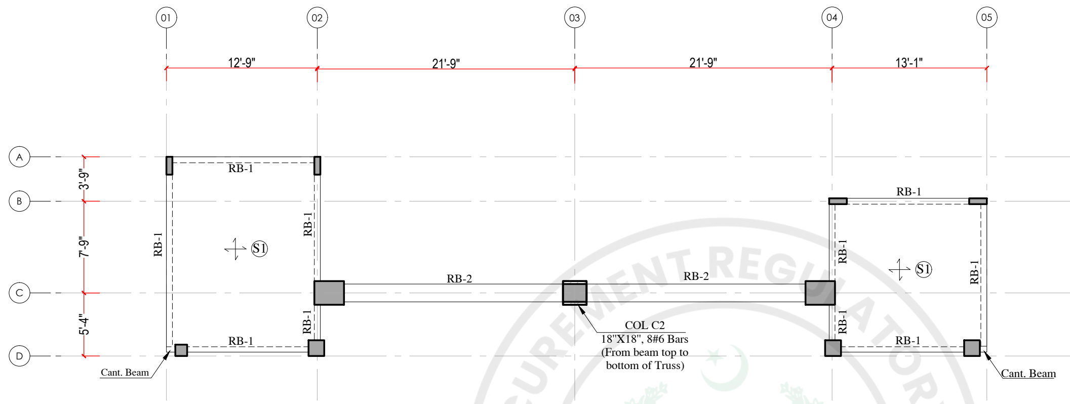
ROOF LEVEL PLAN
