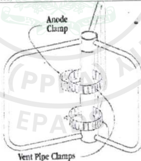
Figure 1: CENTRALIZER FRAME (MS WITH WELDED CLAMPS FOR ANODE AND PVC SLOTTED PIPE)
