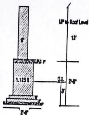
FOUNDATION SECTION
