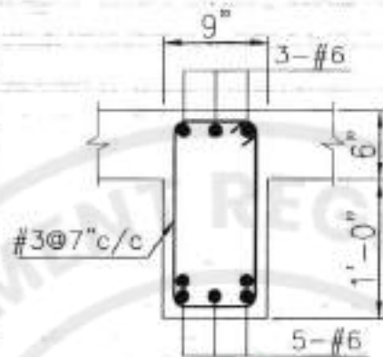
BEAM B-2
