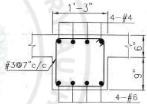
BEAM B-6
