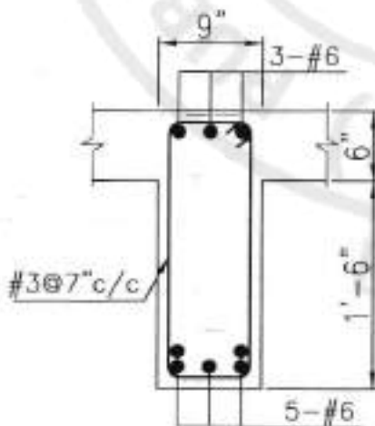
BEAM B-7
