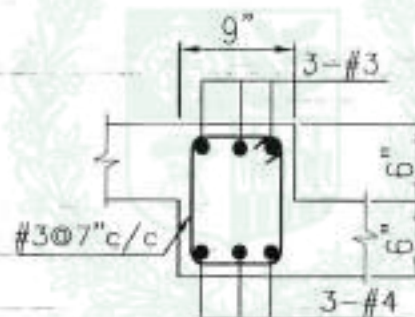
BEAM B-5
