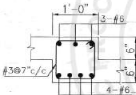
BEAM B-4
