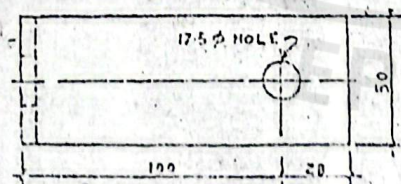
D-SHACKLE STRAP
