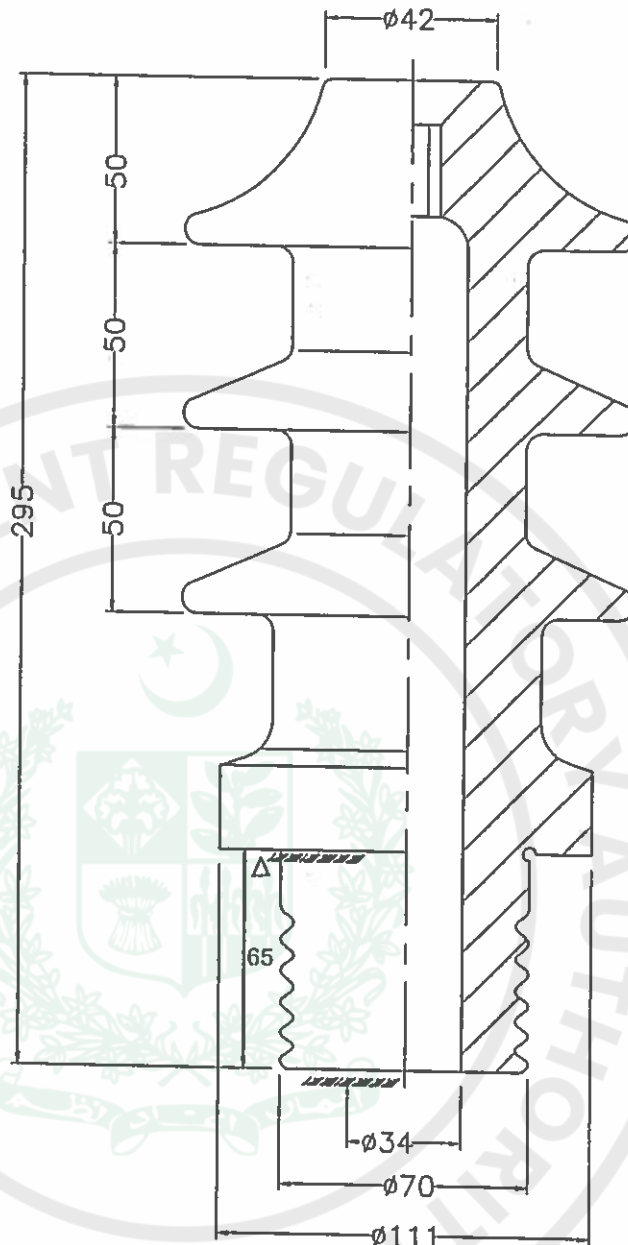
SECTIONAL ELEVATION
