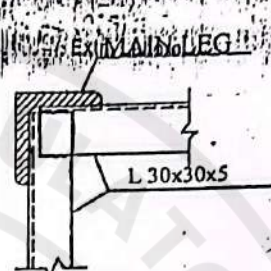
DETAIL OF FRAME JOINTS SECTION "K - K"
