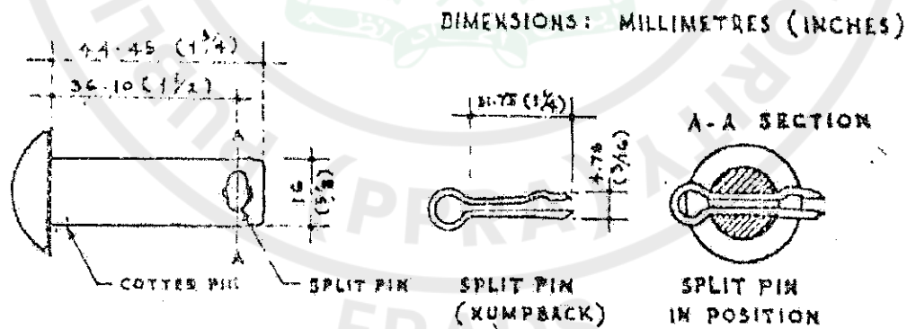
Fig. 2 Cotter Pin and Split Pin
