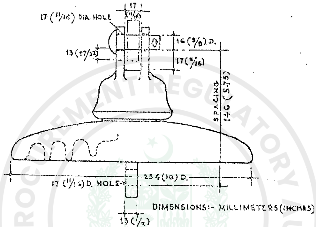
Fig. 1 Standard Clevis and Eye Type Disc Insulator
