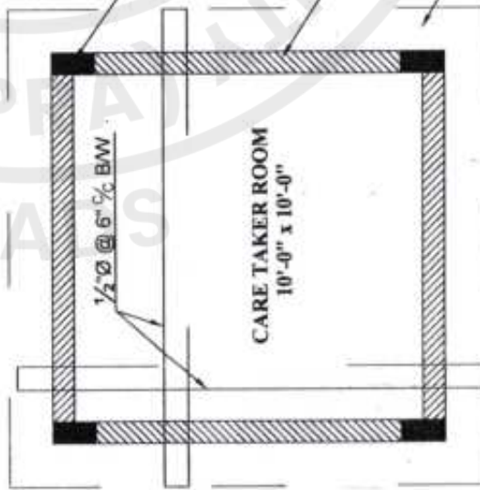
ROOF SLAB
