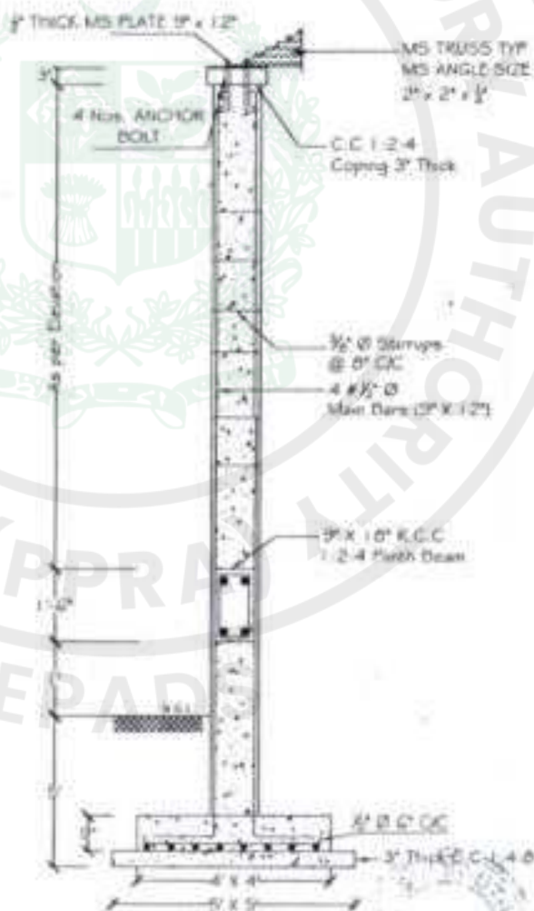
TYPICAL SECTION B-B
