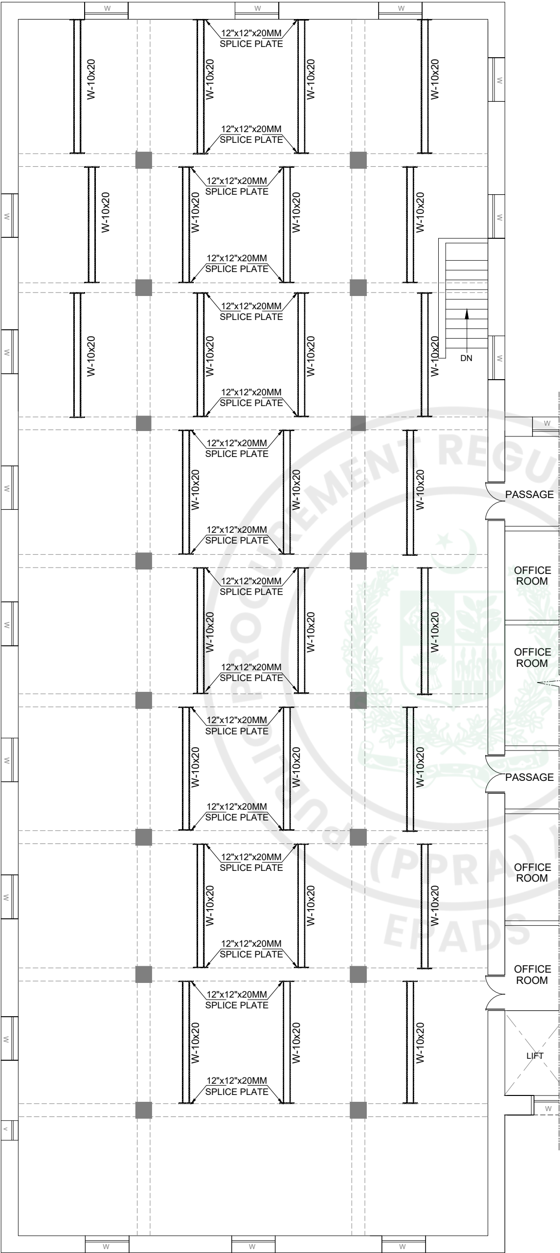
PROPOSED PART PLAN OF 1ST FLOOR BMB
