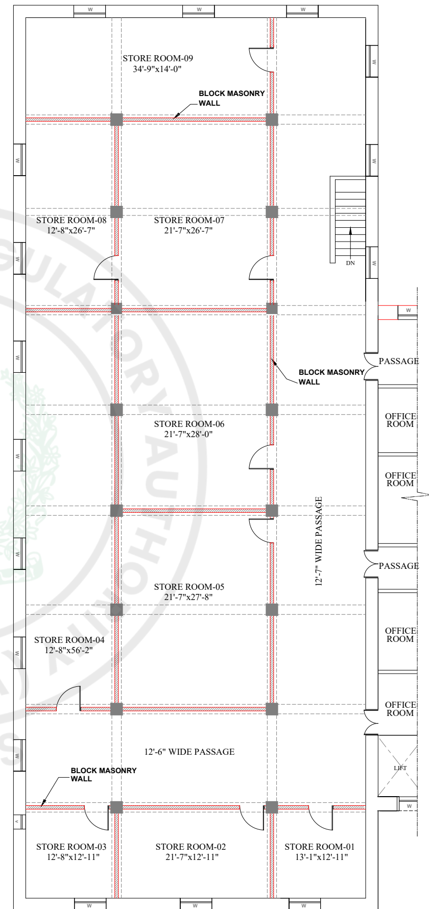
PROPOSED PART PLAN OF 1ST FLOOR BMB BLOCK MASONRY WALL
