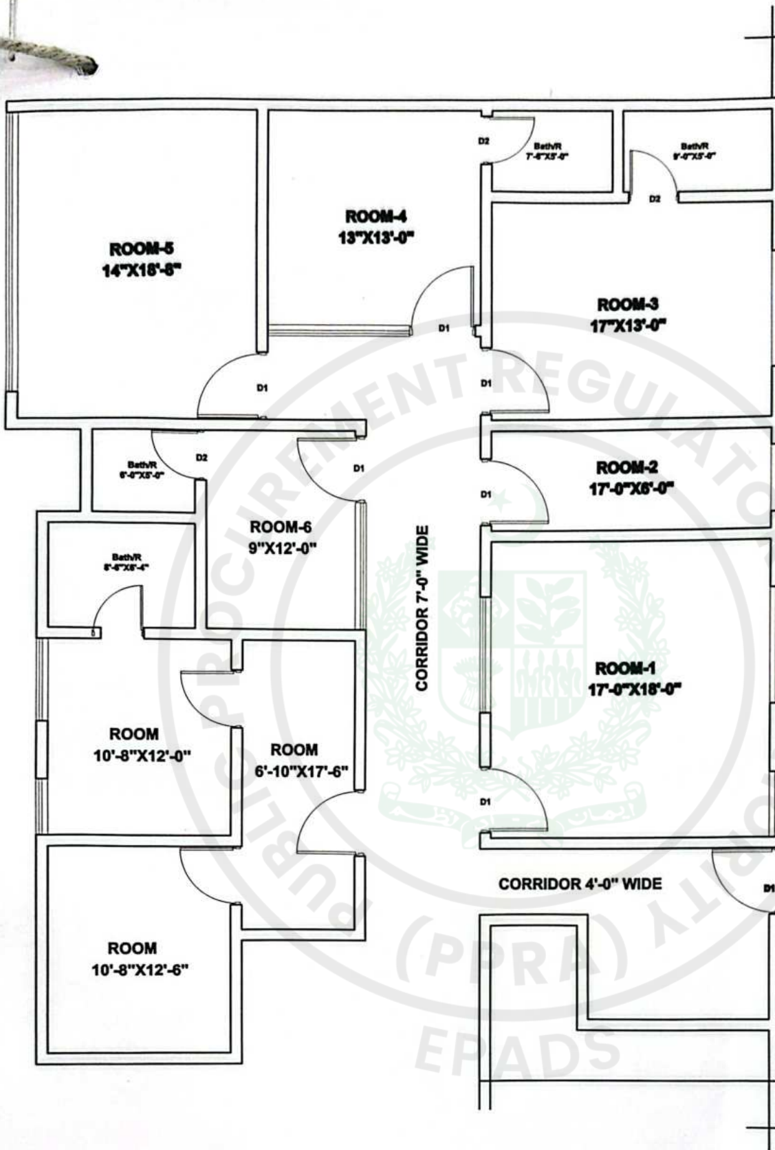
EXISTING FLOOR PLAN OF LAB (CHILAS)
