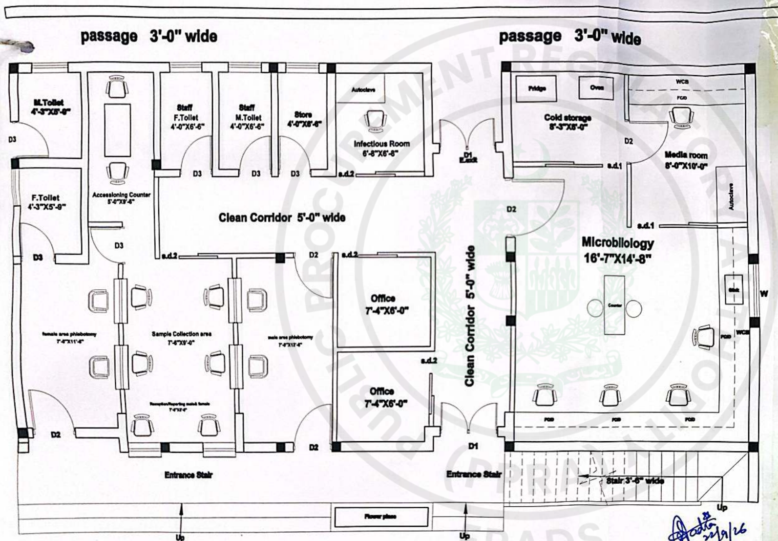
PROPOSED DESIGN OF LAB G.F (GILGIT)
