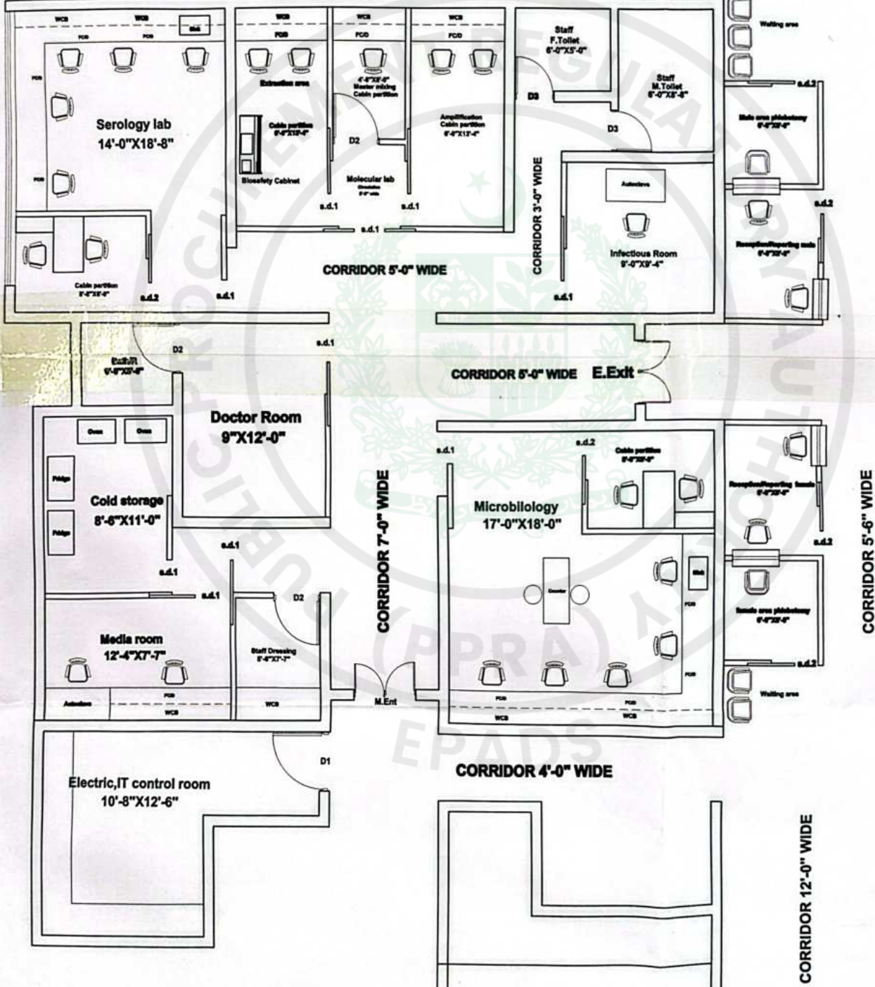
PROPOSED FLOOR PLAN OF LAB (CHILAS)
