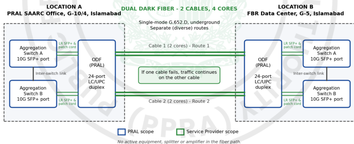
Figure 1: Dual dark fiber link diagram
